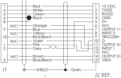
SCHEMATIC
