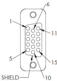
D-SUB END VIEW (J2)
