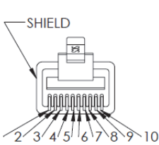
RJ50 END VIEW (J1)
