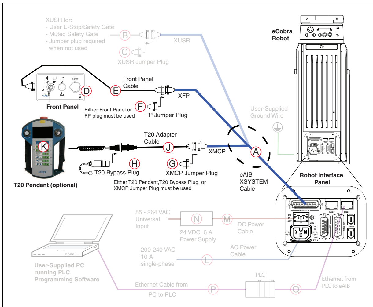
Figure 3-2. Pendant and Front Panel Installation with eCobra Robot and PLC
