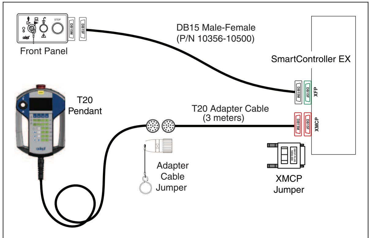
Figure 3-1. Pendant and Front Panel Installation with SmartController EX Motion Controller
