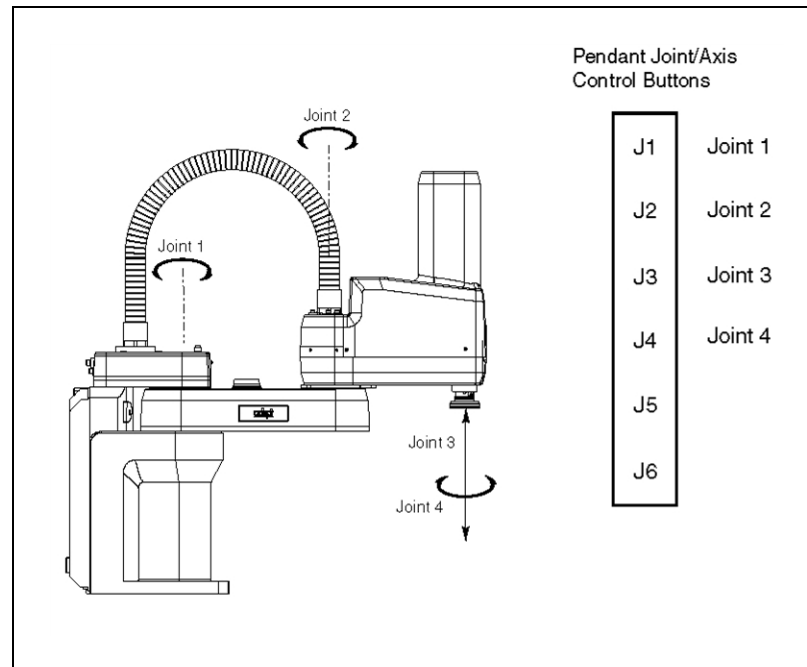
Figure 4-8. Joint Mode (Four-Axis Cobra Robot Shown)
