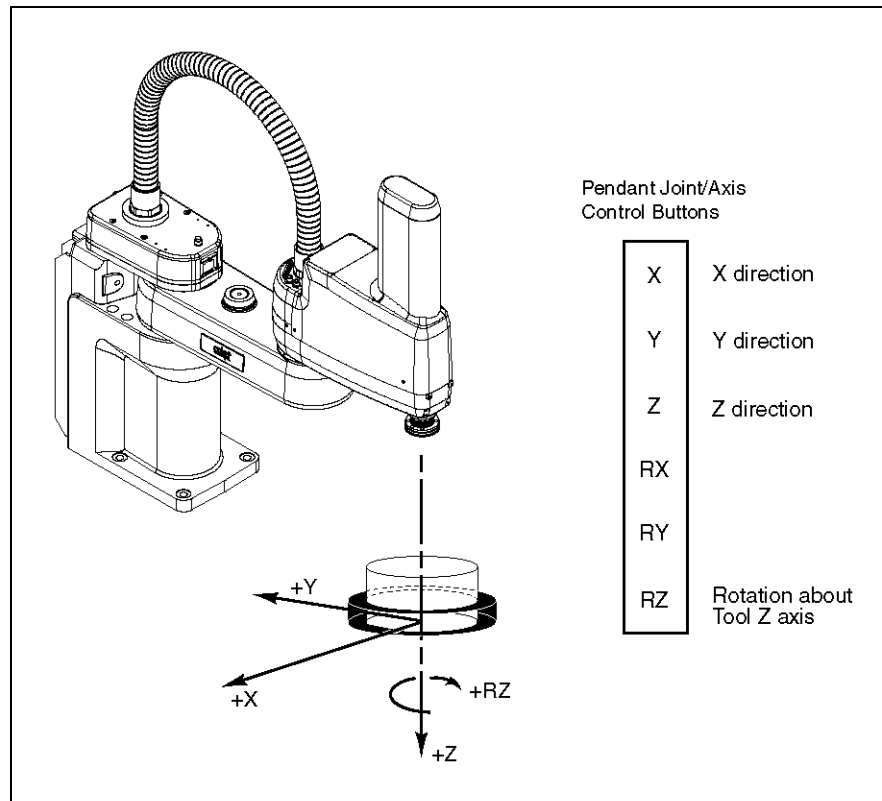
Figure 4-10. Tool Mode (Four-Axis Cobra Robot Shown)
