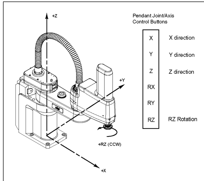
Figure 4-9. World Mode (Four-Axis Cobra Robot Shown)
