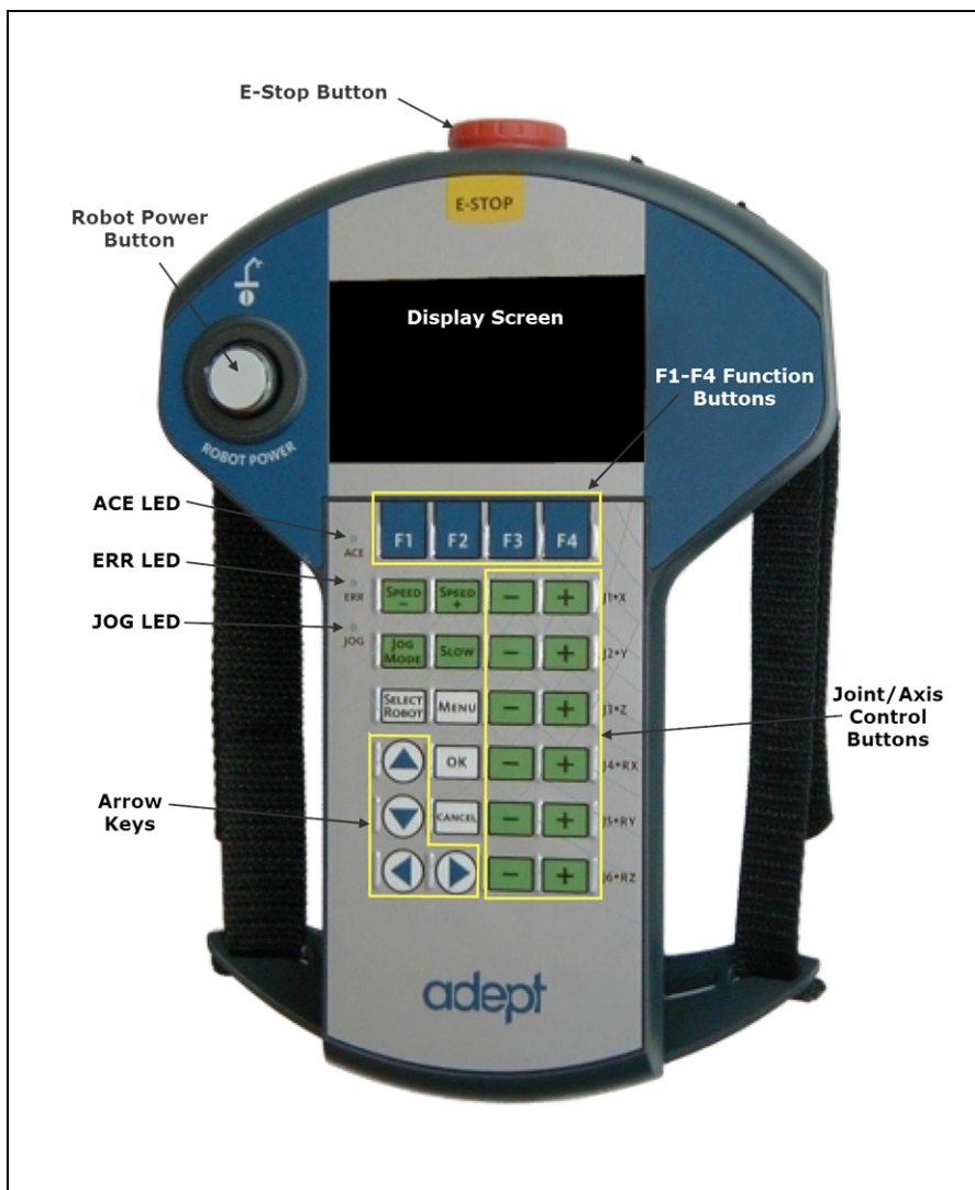
Figure 4-1. T20 Pendant Controls and LEDs
