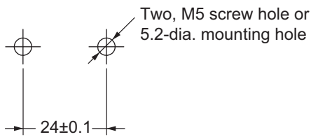
Mounting Hole Dimensions
