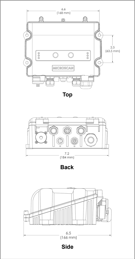
MS-Connect 210 Dimensions
