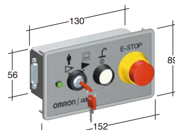
Front panel
