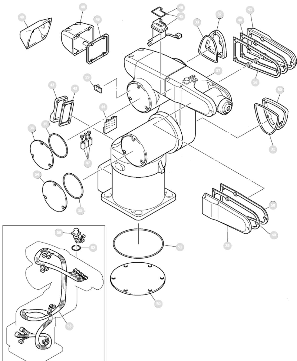
Viper Parts Diagram
